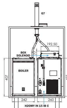
Pro-Stream Hot & Cold
