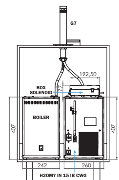
Pro-Stream hot, Cold & Sparkling
